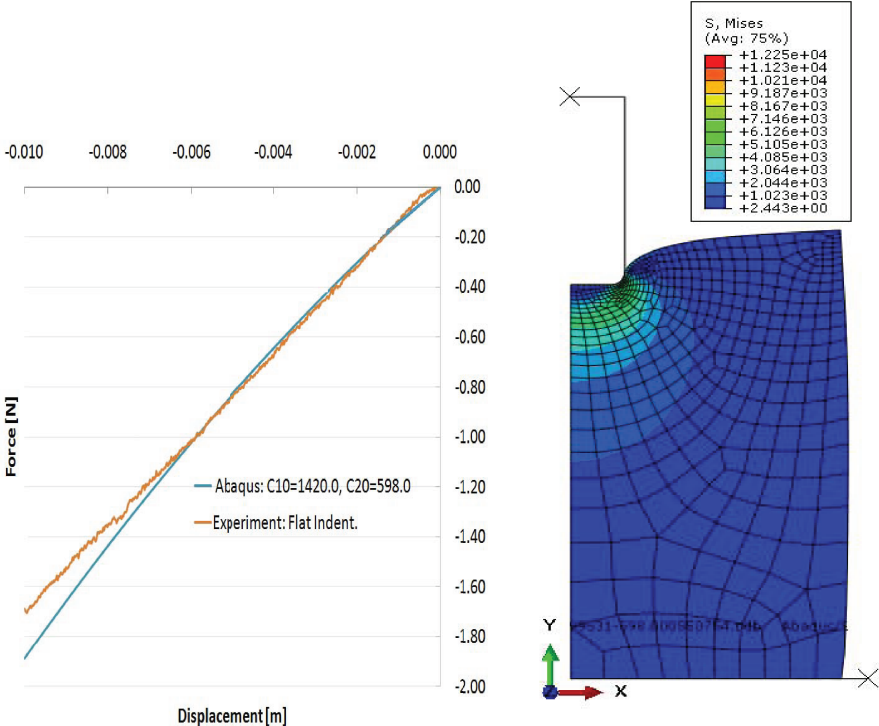
(a) F/D relation with optimal parameters in FEM simulation vs. experiments.
