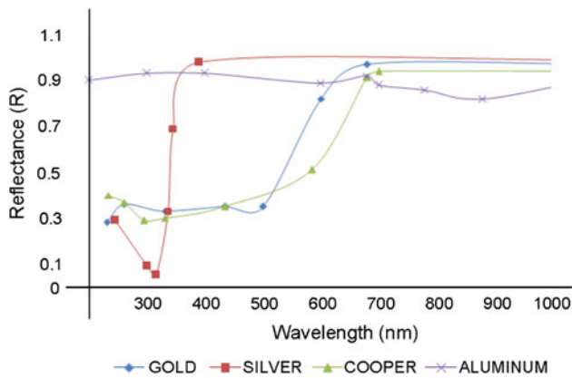
Fig. 2 Reflectance versus wavelength for Au, Ag, Cu and Al [32]
