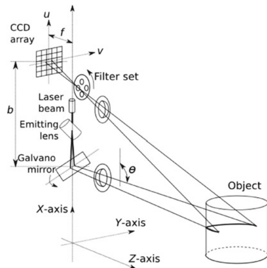
Fig. 1 Triangulation principle and main hardware components of the Vivid 9i system
