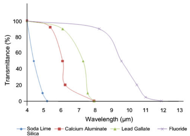
Fig. 3 Transmittance versus wavelength the IR Range [32]
