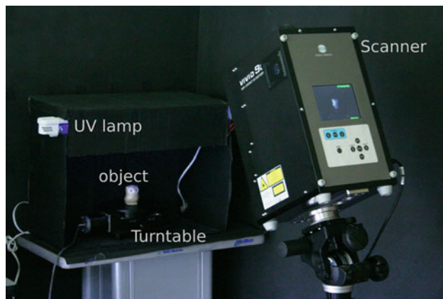
Fig. 4 Acquisition system
